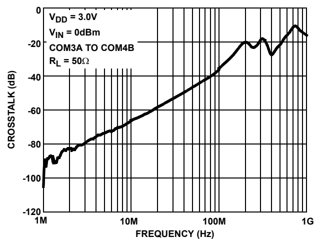
FIGURE 22. CROSSTALK
