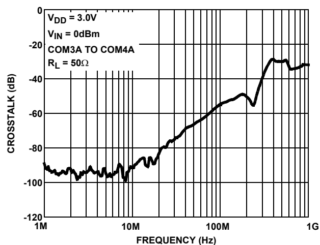
FIGURE 21. CROSSTALK
