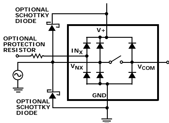
FIGURE 7. OVERVOLTAGE PROTECTION
