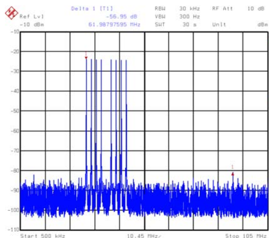
FIGURE 3. EIGHT TONES (CREST FACTOR = 8.9) AT 37MHz, 210MSPS CLOCK, 2.1MHz SPACING (57dBc - NYQUIST)
