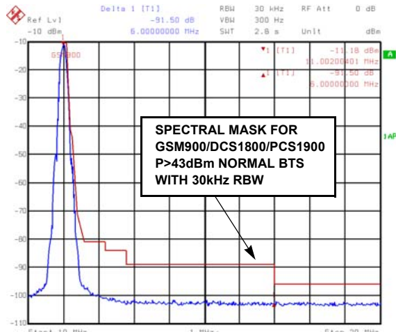
FIGURE 1. EDGE AT 11MHz, 78MSPS CLOCK (91+dBc @ \Delta f = +6 MHz)
