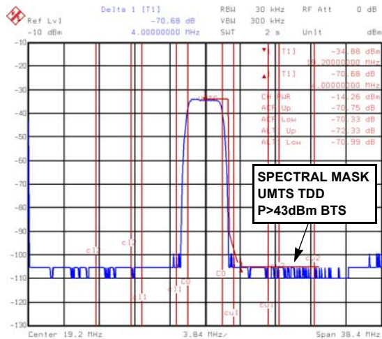
FIGURE 7. UMTS AT 19.2MHz, 76.8MSPS (70dB 1st ACPR, 70dB 2nd ACPR)
