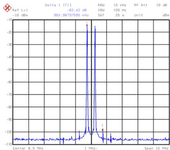
FIGURE 11. TWO TONES (CkHf=6) AT 8.5MHz, 50MSPS CLOCK, 500kHz SPACING (82dBc - 10MHz WINDOW, 6dB PAD)
