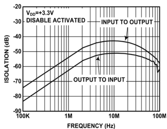
FIGURE 10. ISOLATION vs FREQUENCY
