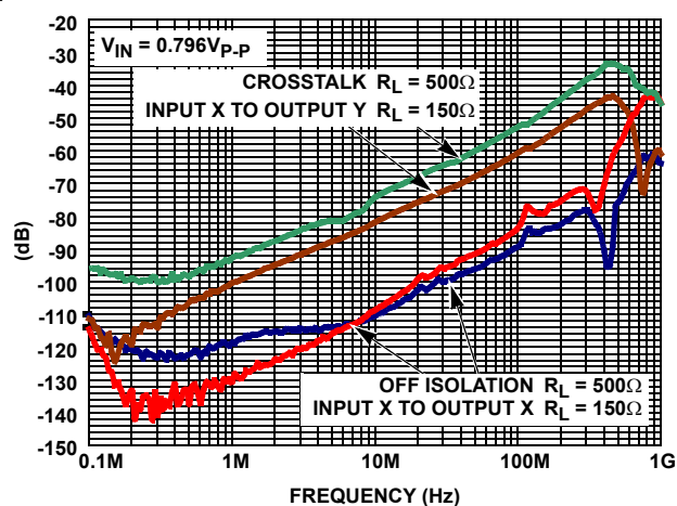
FIGURE 14. MUX2: CROSSTALK AND OFF ISOLATION
