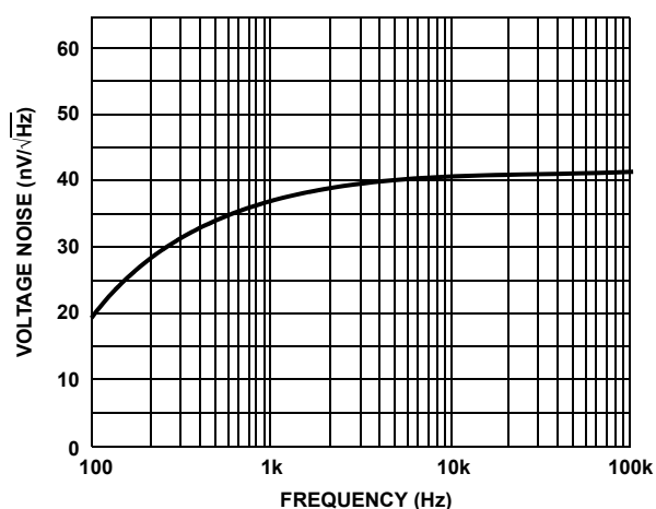
FIGURE 16. MUX2: INPUT NOISE vs FREQUENCY
