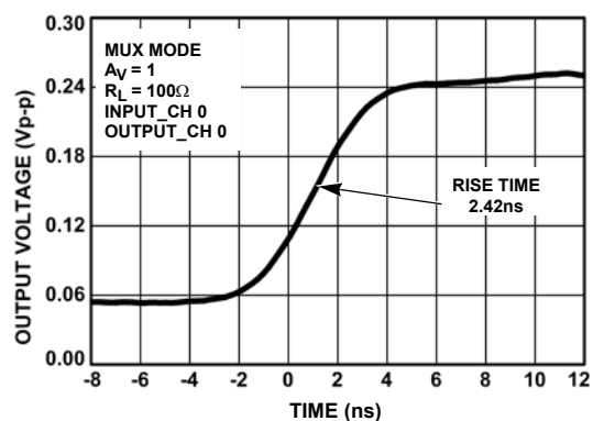
FIGURE 17. RISE TIME - A_V = 1
