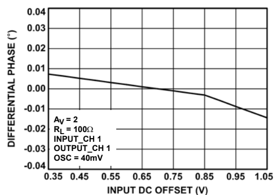
FIGURE 30. DIFFERENTIAL PHASE, A_V = 2
