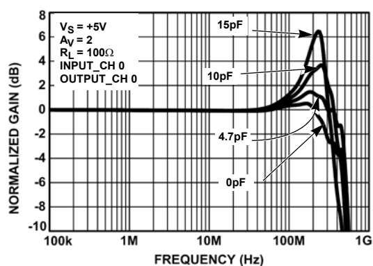
FIGURE 2. FREQUENCY RESPONSE - VARIOUS C_L , A_V = 2 , MUX MODE
