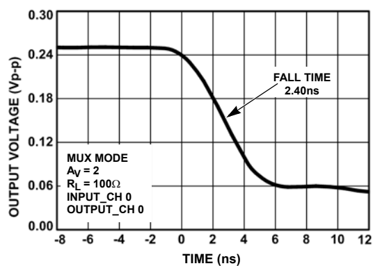
FIGURE 20. FALL TIME - A_V = 2
