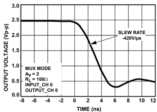
FIGURE 24. FALLING SLEW RATE - A_V = 2
