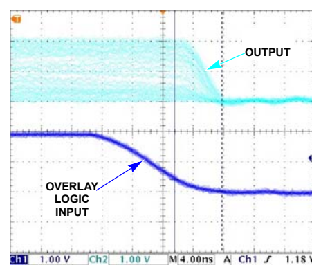
FIGURE 26. OVERLAY SWITCH TURN-OFF DELAY TIME
