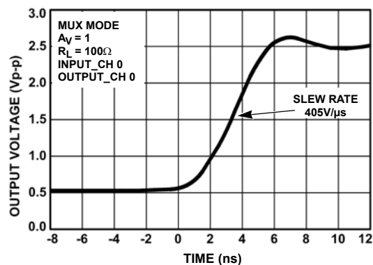
FIGURE 21. RISING SLEW RATE - A_V = 1
