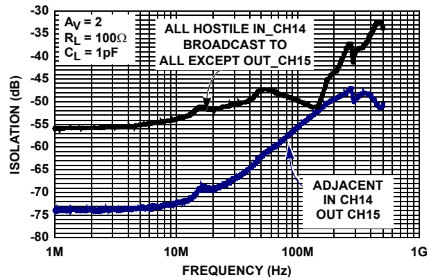
FIGURE 12. CROSSTALK - A_V = 2
