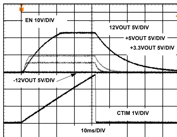
FIGURE 15. ISL6111 TURN-ON INTO M12V OC CONDITION
