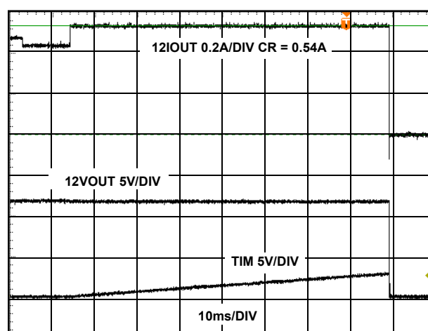
FIGURE 17. 12VOUT INTO CR (VCRSET = 0.461V)
