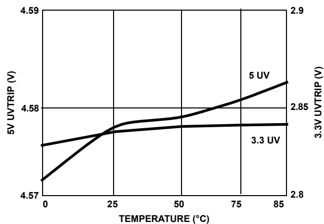
FIGURE 9. UV TRIP vs TEMPERATURE
