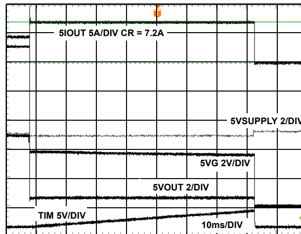
FIGURE 19. 5VOUT INTO CR (VCRSET = 0.461V)
