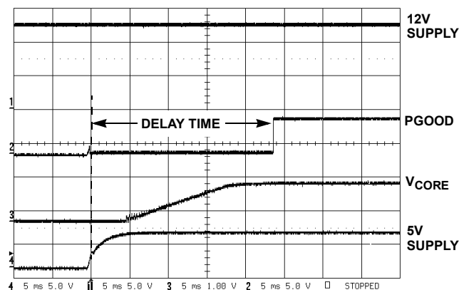
FIGURE 5. SUPPLY POWERED BY ATX SUPPLY
