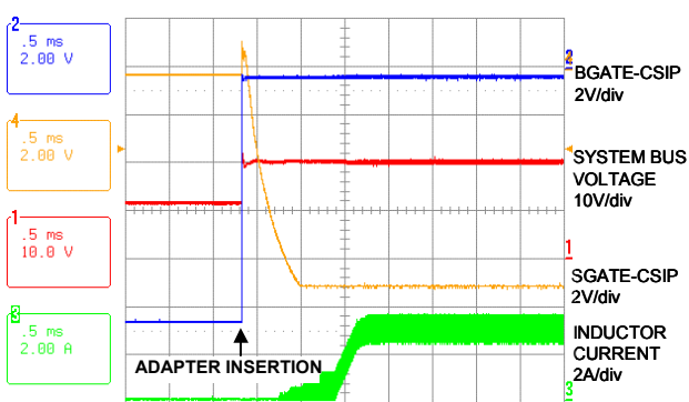
FIGURE 15. AC ADAPTER INSERTION
