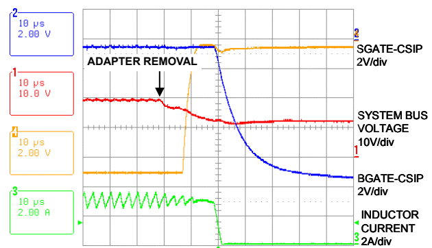
FIGURE 14. AC ADAPTER REMOVAL
