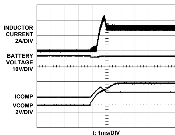
FIGURE 10. BATTERY INSERTION
