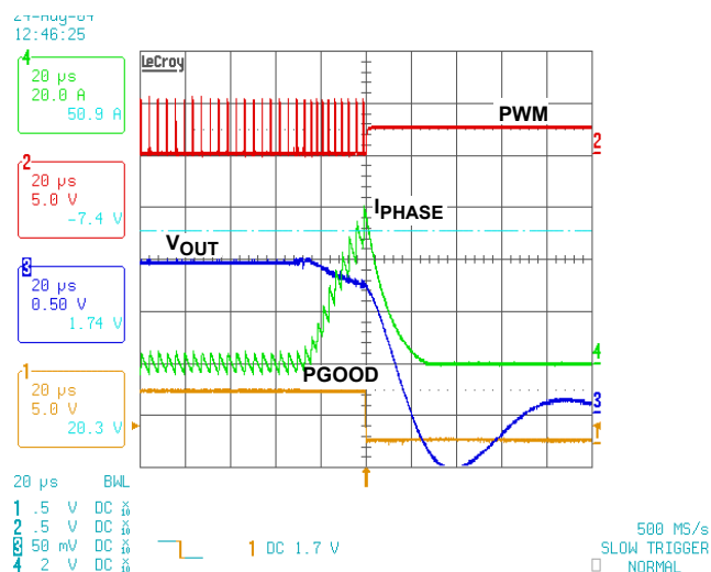
FIGURE 29. WOCP - SHORT CIRCUIT PROTECTION
