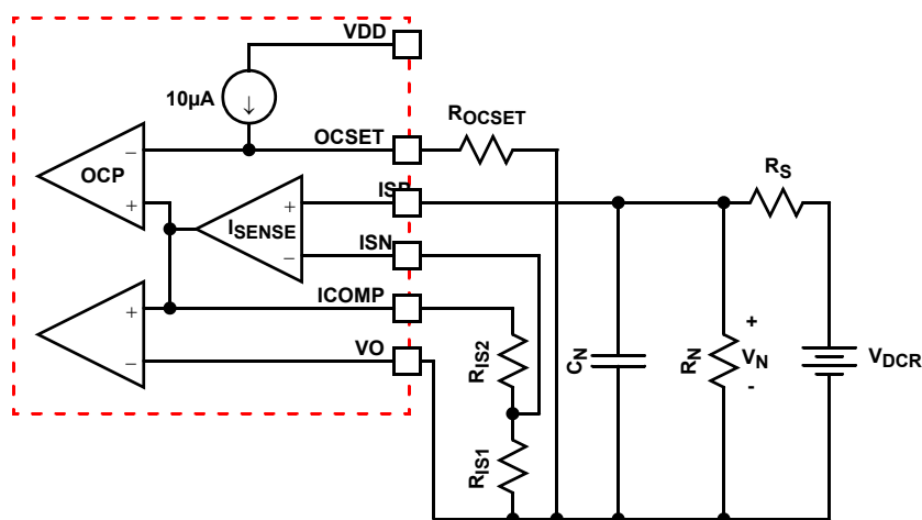
FIGURE 8. EQUIVALENT MODEL OF CURRENT SENSE USING INDUCTOR DCR CURRENT SENSE
