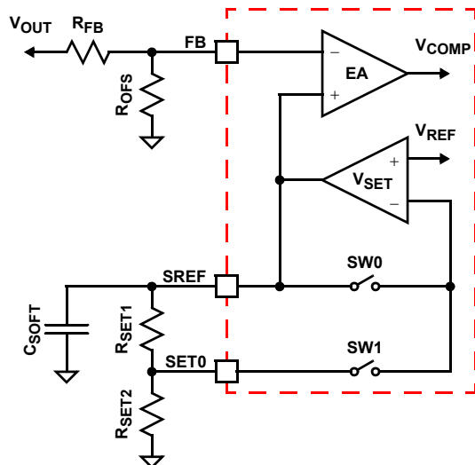
FIGURE 5. ISL62873 VOLTAGE PROGRAMMING CIRCUIT
