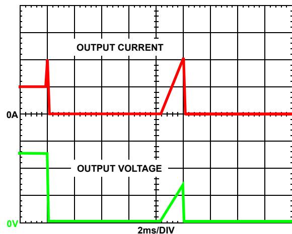
FIGURE 11. OVERCURRENT BEHAVIOR IN HICCUP MODE. F_{SW} = 500\text{kHz}
