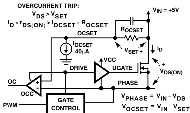
FIGURE 2. OVERCURRENT DETECTION
