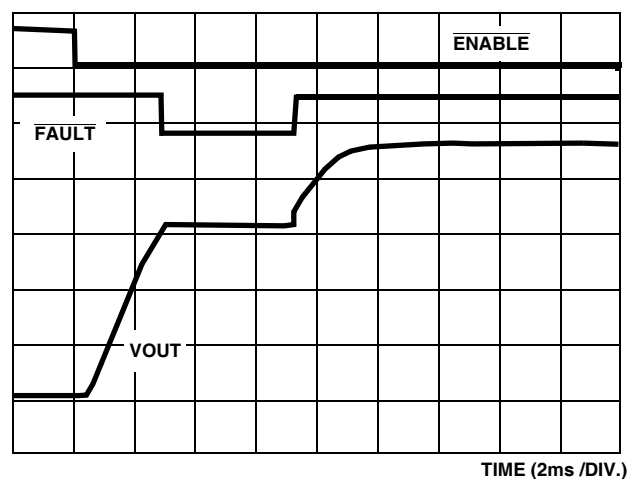
FIGURE 12. VENDOR IC TURN-ON INTO MOMENTARY OC
