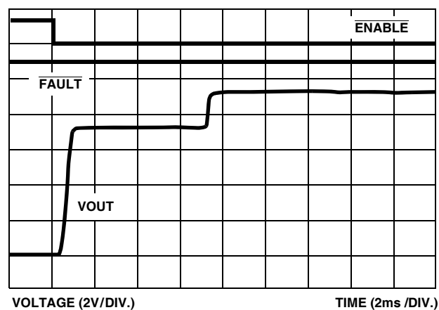
FIGURE 11. ISL6436L TURN-ON INTO 1.5A MOMENTARY OC
