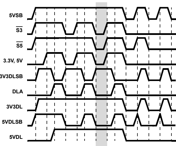
FIGURE 5. 5V DUAL AND 3.3V DUAL /3.3V SB TIMING DIAGRAM; ISL6504A
