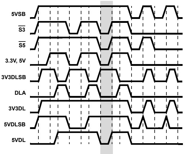
FIGURE 4. 5V DUAL AND 3.3V DUAL /3.3V SB TIMING DIAGRAM; ISL6504
