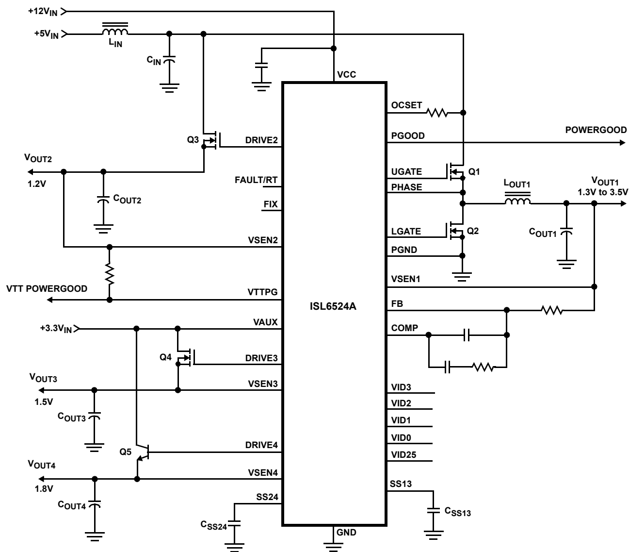
FIGURE 3. TYPICAL APPLICATION
