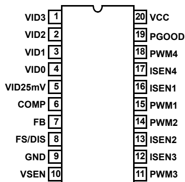
ISL6552CB (20 LEAD SOIC)
