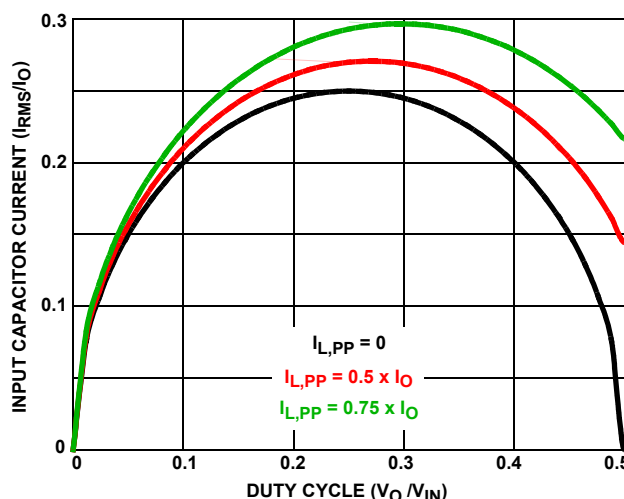
FIGURE 11. NORMALIZED INPUT RMS CURRENT vs DUTY CYCLE FOR A 2-PHASE CONVERTER
