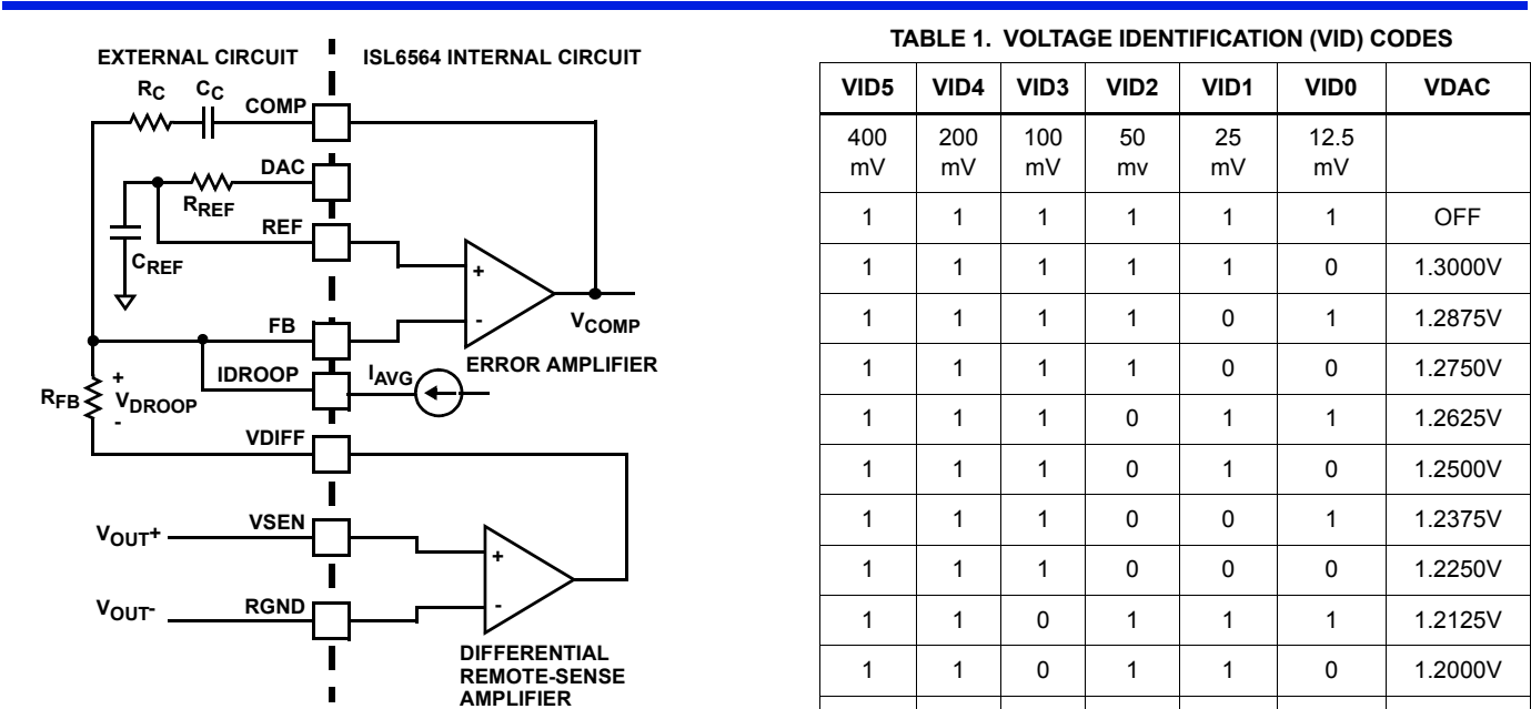
FIGURE 8. OUTPUT VOLTAGE AND LOAD-LINE REGULATION WITH OFFSET ADJUSTMENT
