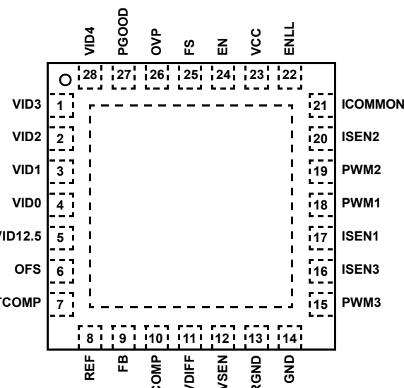
ISL6565BCR (QFN) TOP VIEW
