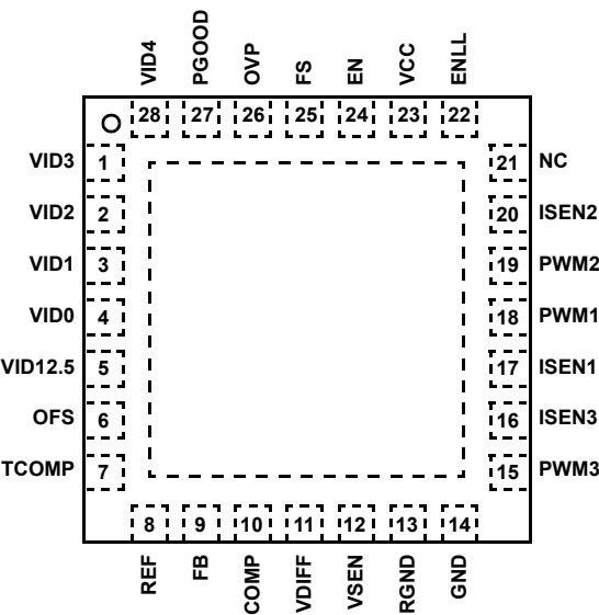
ISL6565ACR (QFN) TOP VIEW
