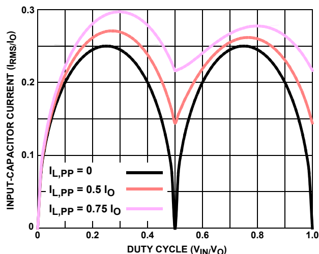
FIGURE 19. NORMALIZED INPUT-CAPACITOR RMS CURRENT FOR 2-PHASE CONVERTER
