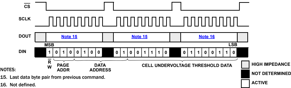
FIGURE 55. SPI FULL DUPLEX (STAND-ALONE) WRITE COMMAND EXAMPLE: WRITE UNDERVOLTAGE THRESHOLD DATA
