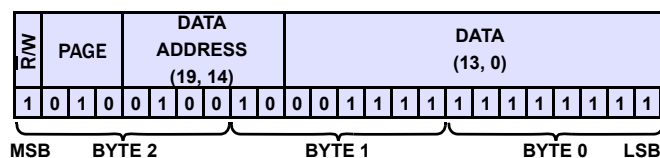
FIGURE 53E. DEVICE WRITE: WRITE EXTERNAL TEMPERATURE LIMIT = 14'h0FFF
