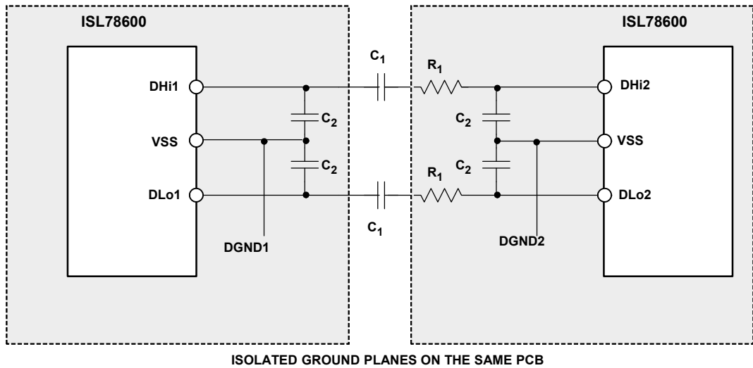
FIGURE 41. ISL78600 DAISY CHAIN – BOARD LEVEL IMPLEMENTATION CIRCUIT
