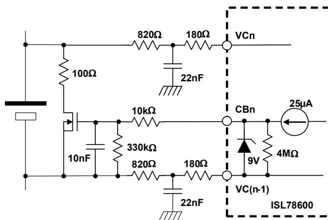
FIGURE 36. ALTERNATE CELL MONITOR AND BALANCE CIRCUIT ARRANGEMENT (VC1 TO VC9)
