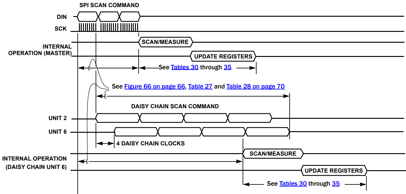
FIGURE 65. MEASUREMENT TIMING (6 DEVICE DAISY CHAIN)
