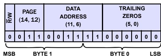
FIGURE 53B. DEVICE LEVEL COMMAND: WAKEUP
