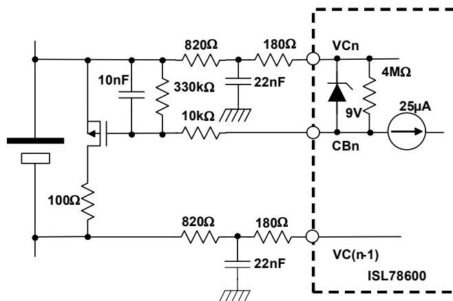
FIGURE 34. ALTERNATE CELL MONITOR AND BALANCE CIRCUIT ARRANGEMENT (VC10 TO VC12)
