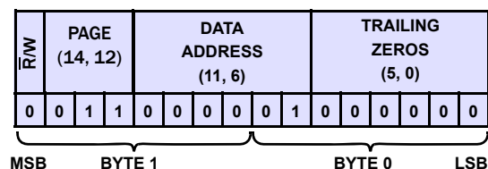
FIGURE 53C. DEVICE LEVEL COMMAND: SCAN VOLTAGES
