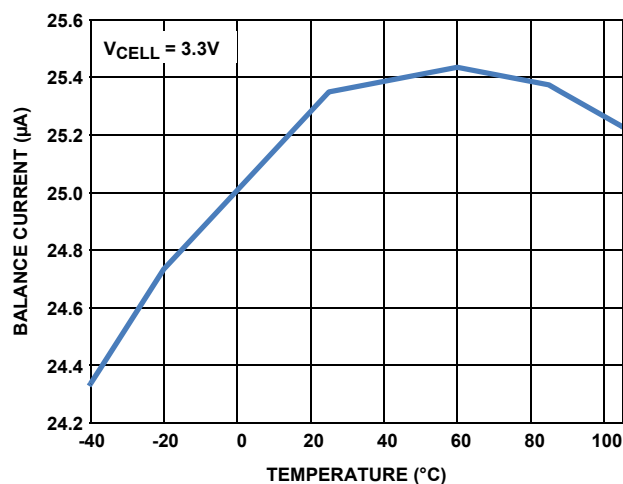
FIGURE 13. BALANCE CURRENT vs TEMPERATURE
