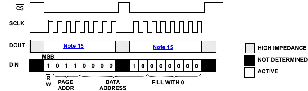
FIGURE 54. SPI FULL DUPLEX (STAND-ALONE) MEASURE COMMAND EXAMPLE: EXT4 VOLTAGE
