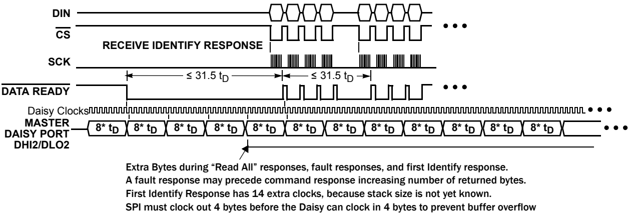
FIGURE 57. EXAMPLE WORST CASE TIMING TO AVOID DAISY BUFFER OVERFLOW
