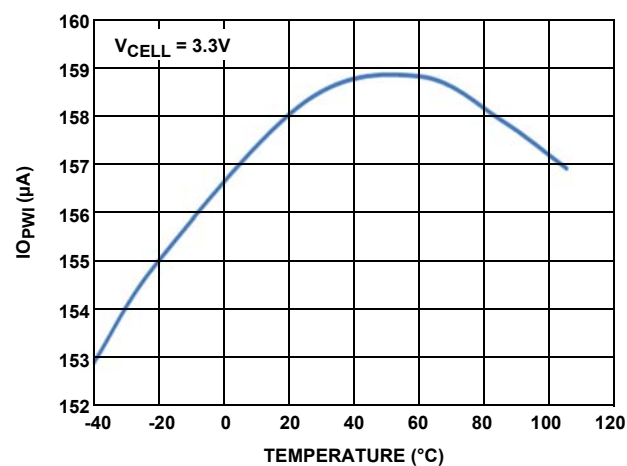
FIGURE 16. OPEN-WIRE TEST CURRENT vs TEMPERATURE (150µA SETTING)
