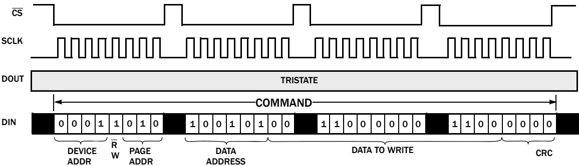
FIGURE 61. SPI HALF DUPLEX (DAISY CHAIN) WRITE REGISTER COMMAND EXAMPLE: WRITE DEVICE 1, DEVICE SETUP REGISTER
