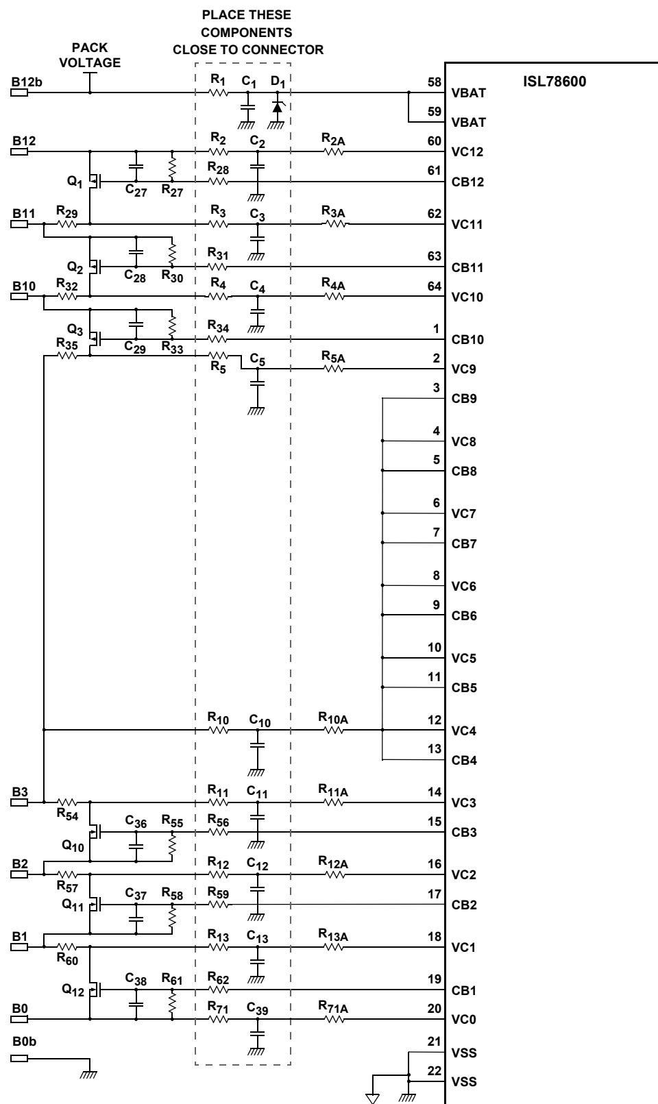
FIGURE 49. TYPICAL APPLICATIONS CIRCUIT – BATTERY CONNECTION CIRCUITS, SYSTEM WITH 6 CELLS
