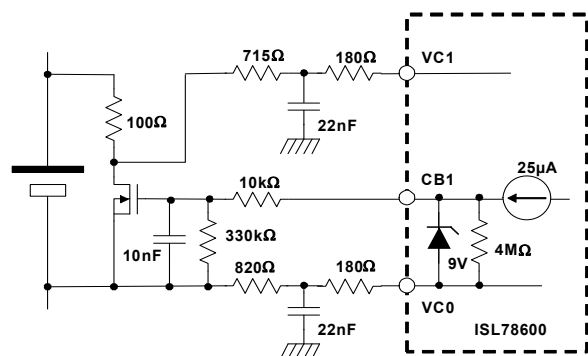
FIGURE 35. CELL MONITOR AND BALANCE CIRCUIT ARRANGEMENT (VC1)
