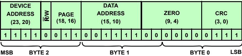
FIGURE 62B. DEVICE LEVEL COMMAND: WAKEUP
