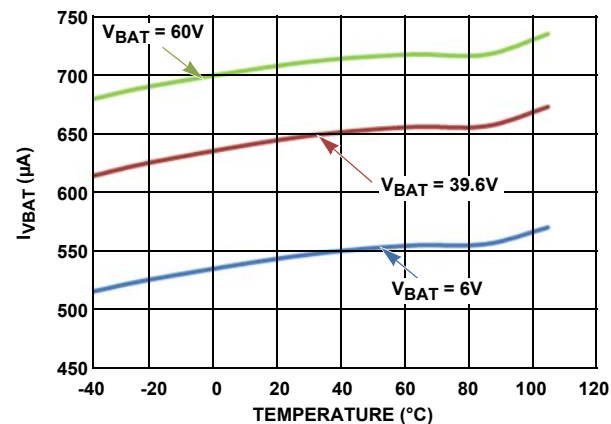
FIGURE 23D. PACK VOLTAGE SUPPLY CURRENT vs TEMPERATURE AT 6V, 39.6V, 60V (DAISY CHAIN TOP)
