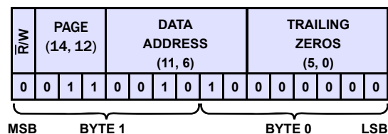
FIGURE 53A. DEVICE LEVEL COMMAND: SLEEP
