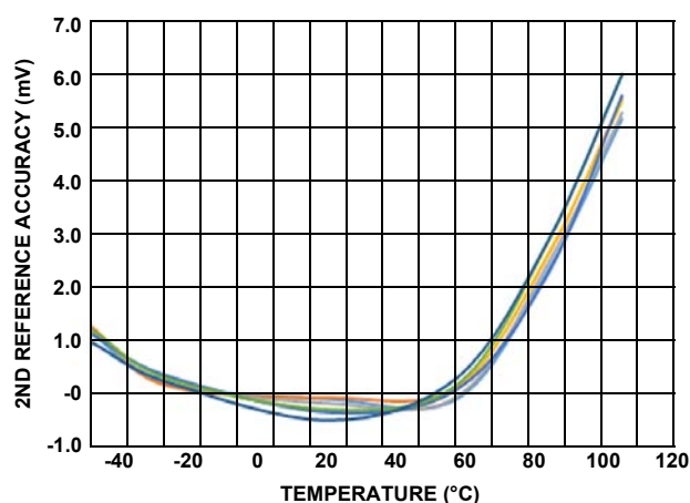
FIGURE 11. VOLTAGE REFERENCE CHECK FUNCTION vs TEMPERATURE ( V_{BAT} = 6V TO 54V )
