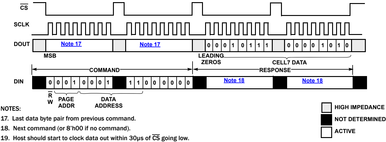
FIGURE 56. SPI FULL DUPLEX (STAND-ALONE) READ COMMAND EXAMPLE: READ CELL 7 DATA
