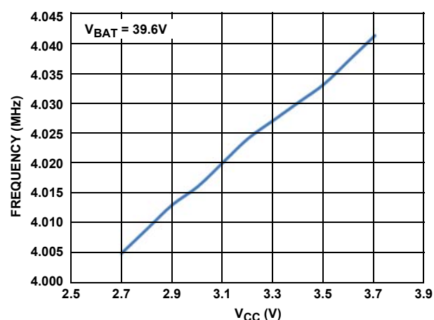
FIGURE 19. 4MHz OSCILLATOR FREQUENCY vs VCC
