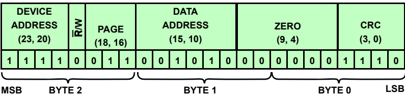
FIGURE 62A. DEVICE LEVEL COMMAND: SLEEP
