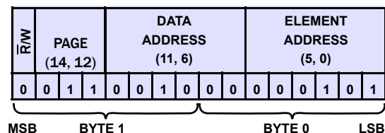
FIGURE 53D. DEVICE LEVEL COMMAND: MEASURE CELL 5 VOLTAGE
