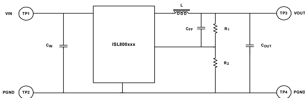
FIGURE 1. BLOCK DIAGRAM
