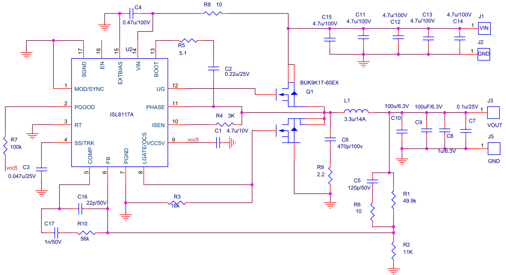
FIGURE 6. ISL8117ADEM01Z SCHEMATIC
