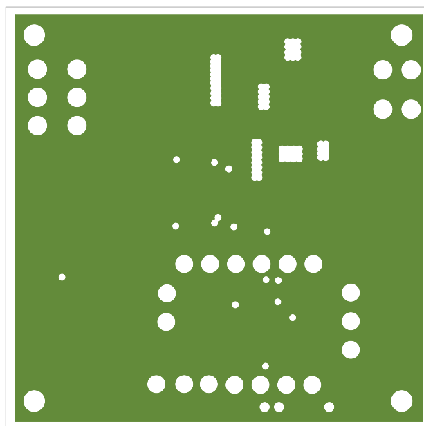
FIGURE 26. THIRD LAYER
