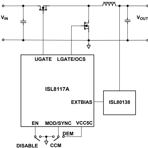
FIGURE 1. BLOCK DIAGRAM
