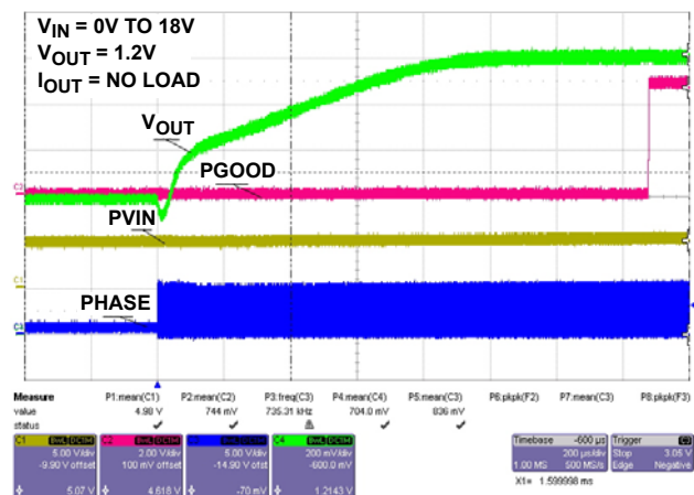
FIGURE 16. 50% PRE-BIAS START UP
