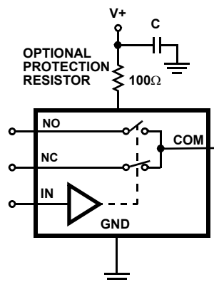
FIGURE 8. V+ SERIES RESISTOR FOR ENHANCED ESD AND LATCH-UP IMMUNITY
