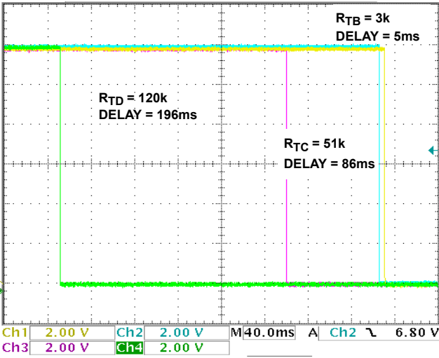
FIGURE 9. ENABLE_X TO ENABLE_X DISABLING
