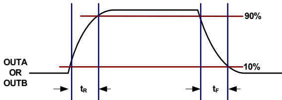
FIGURE 4. RISE/FALL TIMES
