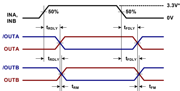
* Logic levels: A option = 3.3V, B option = 5.0V FIGURE 3. PROP DELAYS AND MATCHING
