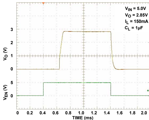
FIGURE 12. TURN ON/TURN OFF RESPONSE
