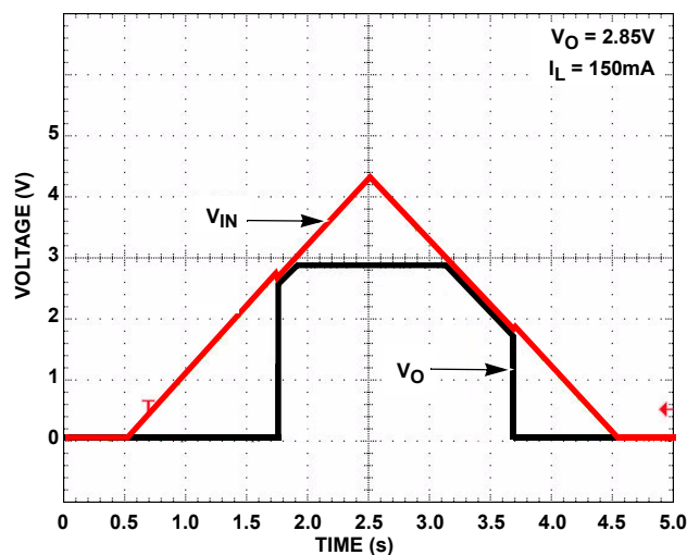
FIGURE 11. POWER-UP/POWER-DOWN
