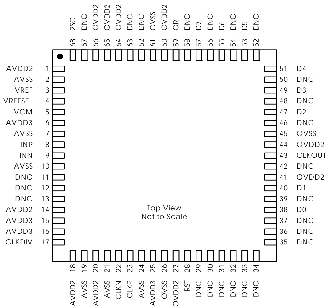
FIGURE 2. PIN CONFIGURATION
