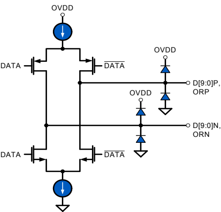
FIGURE 30. LVDS OUTPUTS
