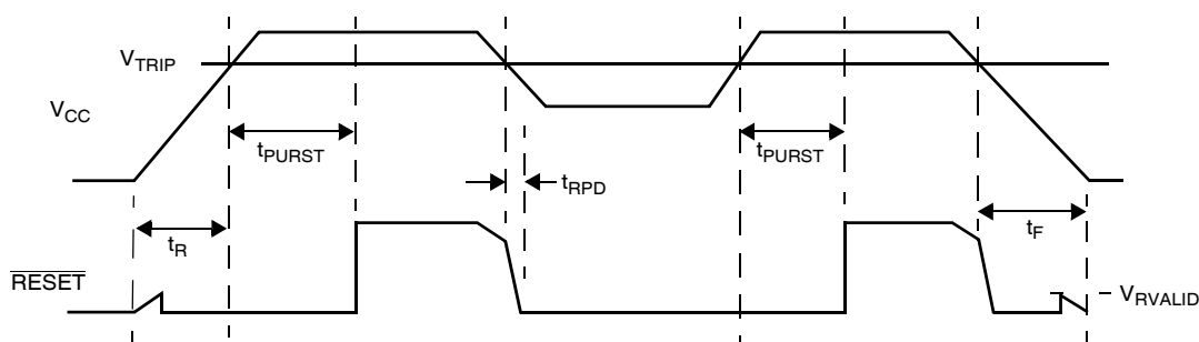
Figure 4. Power-on Reset and Low Voltage Reset
