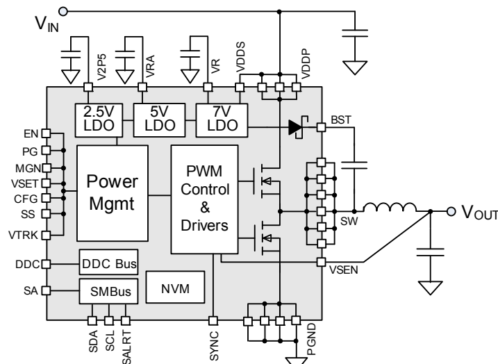
FIGURE 3. BLOCK DIAGRAM
