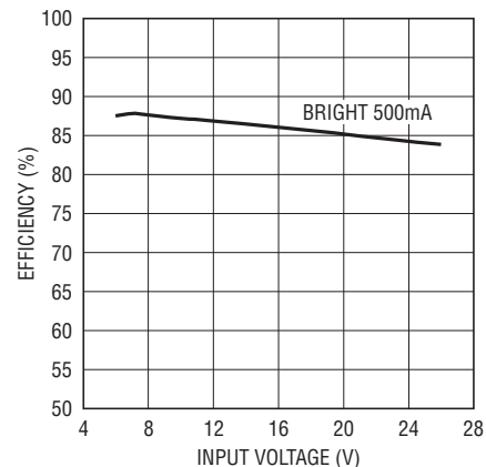
Efficiency for 2 Red LEDs, L = 10μH, 900kHz
