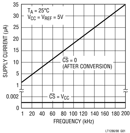
Figure 5. Shutdown current with \overline{\text{CS}} high is 1nA typically, regardless of the clock. Shutdown current with \overline{\text{CS}} = \text{ground} varies from 1µA at 1kHz to 35µA at 200kHz.
