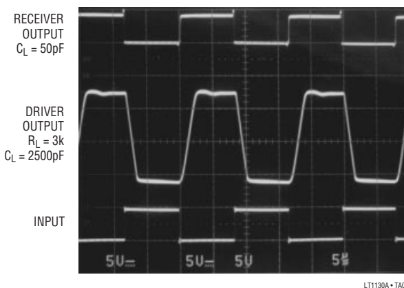
Output Waveforms
