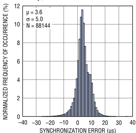
TIMEs Synchronization Error 0 Packet/s Publishing Rate, 1 Hop, 8°C/Min
