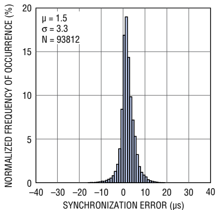
TIMEs Synchronization Error 0 Packet/s Publishing Rate, 1 Hop, 2°C/Min
