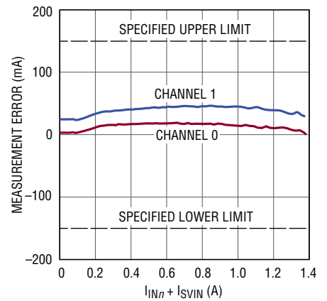
MFR_READ_IIN n (Input Current Readback) Error vs (\text{I}_{\text{VIN}n} + \text{I}_{\text{SVIN}}) , \text{MFR\_PWM\_MODE}_n[1:0] = 10_{\text{b}} , \text{I}_{\text{OUT}n} Swept from 0\text{A} to 13\text{A} , One Channel at a Time, \text{RUN}_{1-n} = 0\text{V}
