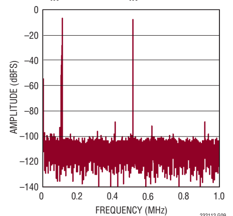
8k Point FFT, IMD, f_S = 2\text{Msps} , V_{IN}^+ = 100\text{kHz} , V_{IN}^- = 500\text{kHz}
