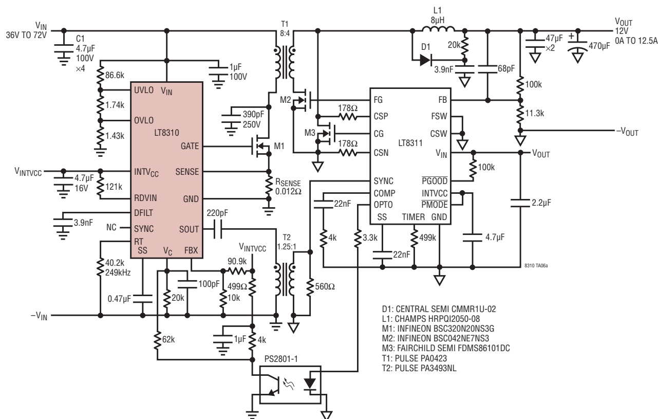
94% Efficient, 150W Isolated Synchronous Forward Converter
