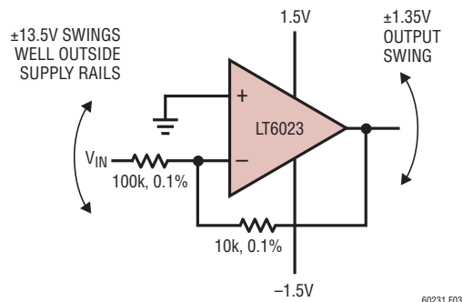
Figure 3. Extreme Inverting Case: Circuit Operates Properly with Input Voltage Swing Well Outside Op Amp Supply Rails
