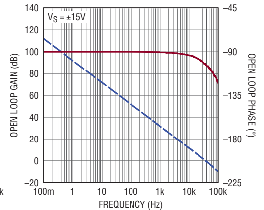
Open-Loop Gain and Phase vs Frequency
