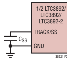
Figure 5. Using the TRACK/SS Pin to Program Soft-Start
