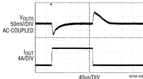
FIGURE 69 CIRCUIT AT 12V_{IN} 0A TO 10A LOAD STEP AT 10A/\mu s
