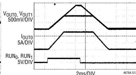
FIGURE 69 CIRCUIT AT 12V_{IN} , 77m\Omega LOAD ON V_{OUT0} , NO LOAD ON V_{OUT1} . T_{ON\_RISE0} = 3ms , T_{ON\_RISE1} = 5.297ms , T_{OFF\_DELAY1} = 0ms , T_{OFF\_DELAY0} = 2.43ms , T_{OFF\_FALL1} = 5.328ms , T_{OFF\_FALL0} = 3ms , ON\_OFF\_CONFIG_7 = 0x1E
