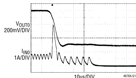
FIGURE 69 CIRCUIT AT 12V_{IN} , 77m\Omega LOAD ON V_{OUT0} PRIOR TO APPLICATION OF SHORT CIRCUIT
