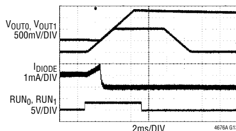
FIGURE 69 CIRCUIT AT 12V_{IN} , 77m\Omega LOAD ON V_{OUT0} , 500\Omega ON V_{OUT1} . V_{OUT1} PRE-BIASED THROUGH A DIODE. T_{ON\_RISE0} = 3ms , T_{ON\_RISE1} = 5.297ms , T_{OFF\_DELAY1} = 0ms , T_{OFF\_DELAY0} = 2.43ms , T_{OFF\_FALL1} = 5.328ms , T_{OFF\_FALL0} = 3ms , ON\_OFF\_CONFIG_1 = 0x1F , ON\_OFF\_CONFIG_0 = 0x1E
