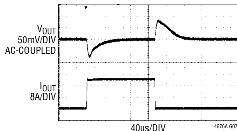
FIGURE 35 CIRCUIT AT 12V_{IN} , INTV_{CC} PIN OPEN CIRCUIT AND V_{OUT\_COMMAND} SET TO 1.000V . 0A TO 20A LOAD STEP AT 20A/\mu s
