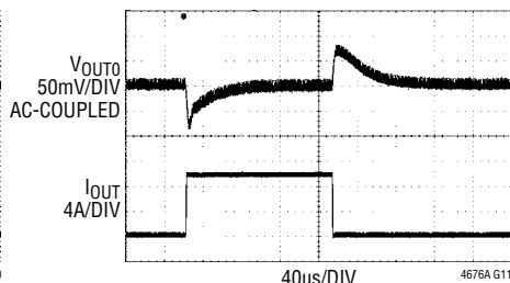
FIGURE 69 CIRCUIT AT 24V_{IN} , C_{OUT0} = 5 \times 100\mu F AND V_{OUT0} COMMANDED TO 3.300V . 0A TO 10A LOAD STEP AT 10A/\mu s
