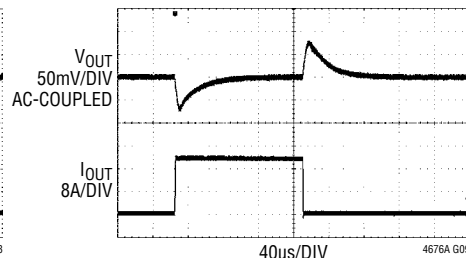
FIGURE 35 CIRCUIT AT 5V_{IN} , V_{OUT\_COMMAND} SET TO 1.000V . 0A TO 20A LOAD STEP AT 20A/\mu s
