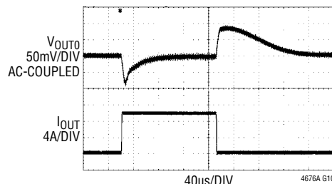
FIGURE 69 CIRCUIT AT 24V_{IN} 0A TO 10A LOAD STEP AT 10A/\mu s
