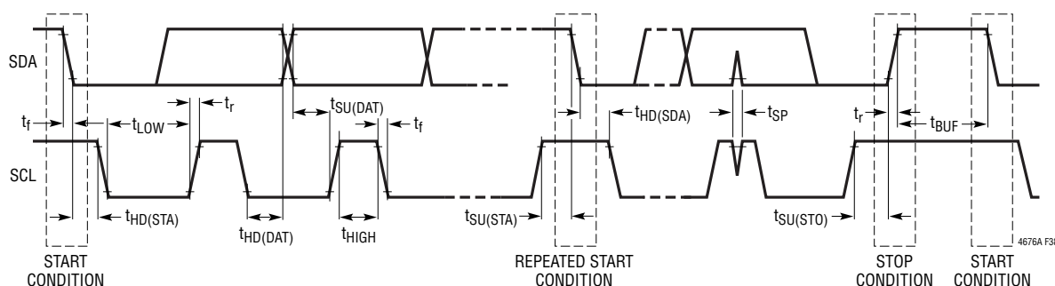
Figure 44. Timing Diagram
