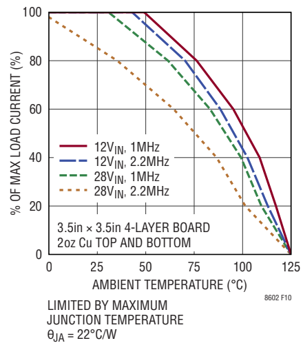
Figure 10. Thermal Derating, I-Grade
