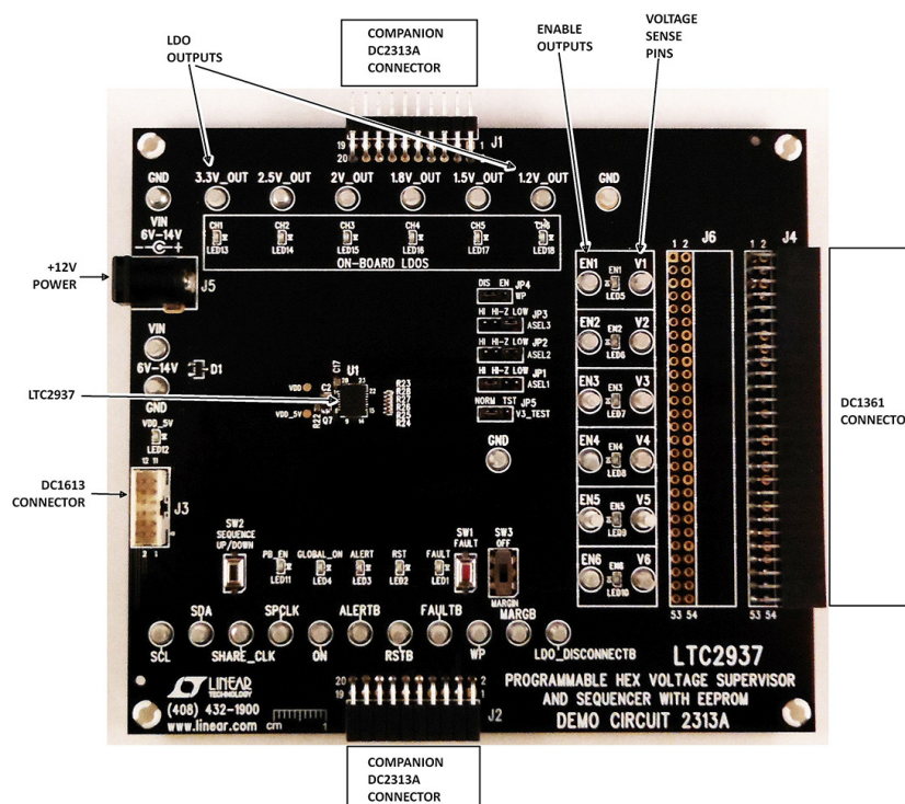
Figure 1. DC2313A Board
